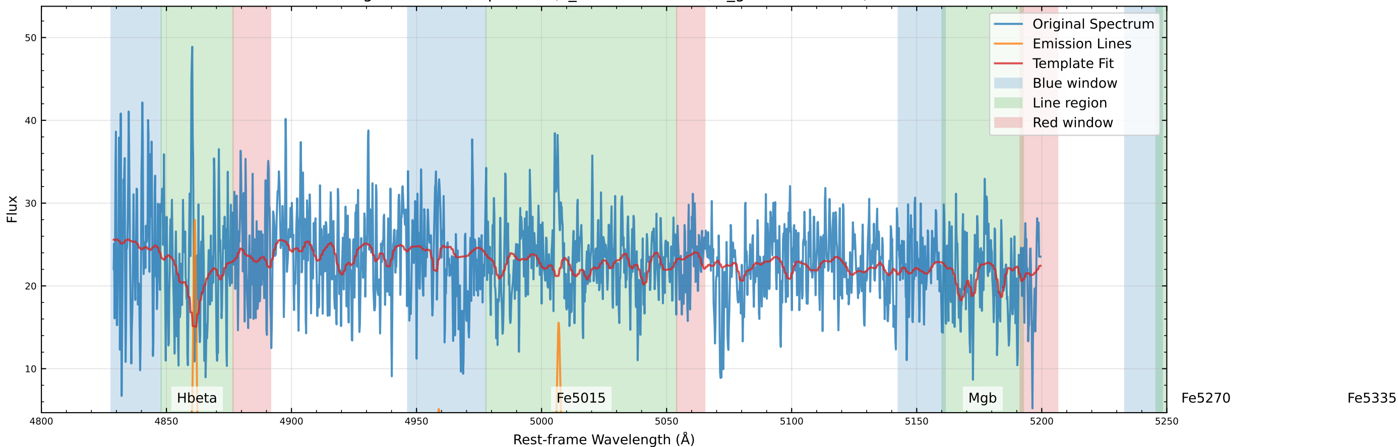
Original Data Comparison (v_star=-58.5 km/s, v_gas=-71.4 km/s)
