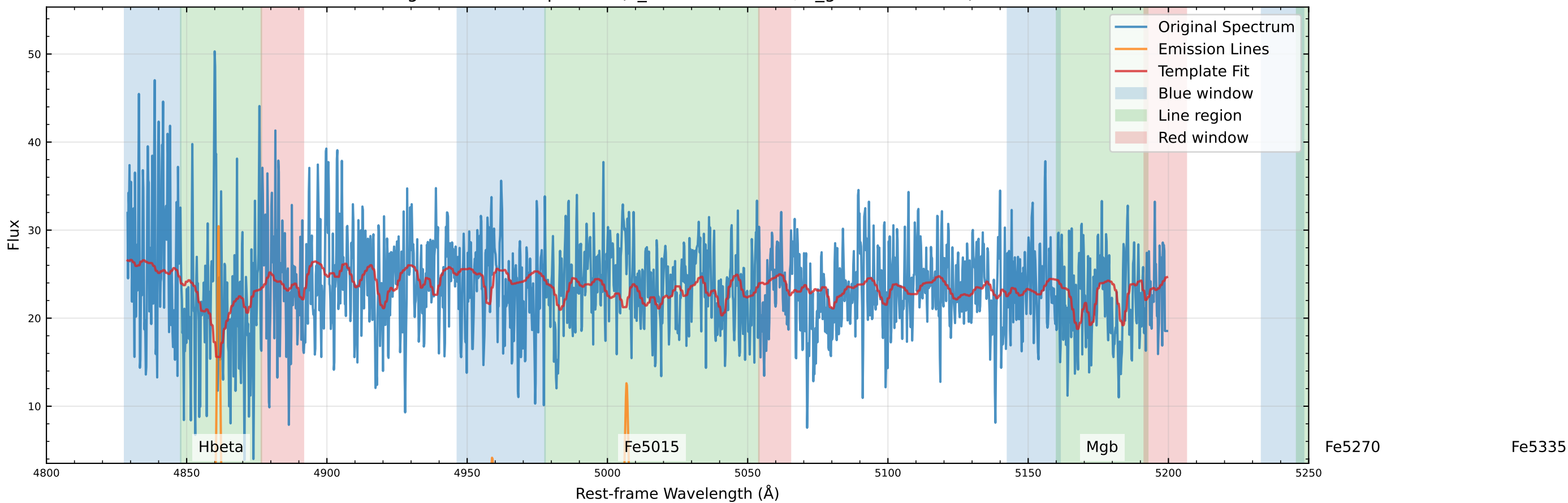
Original Data Comparison (v_star=-90.4 km/s, v_gas=-80.7 km/s)
