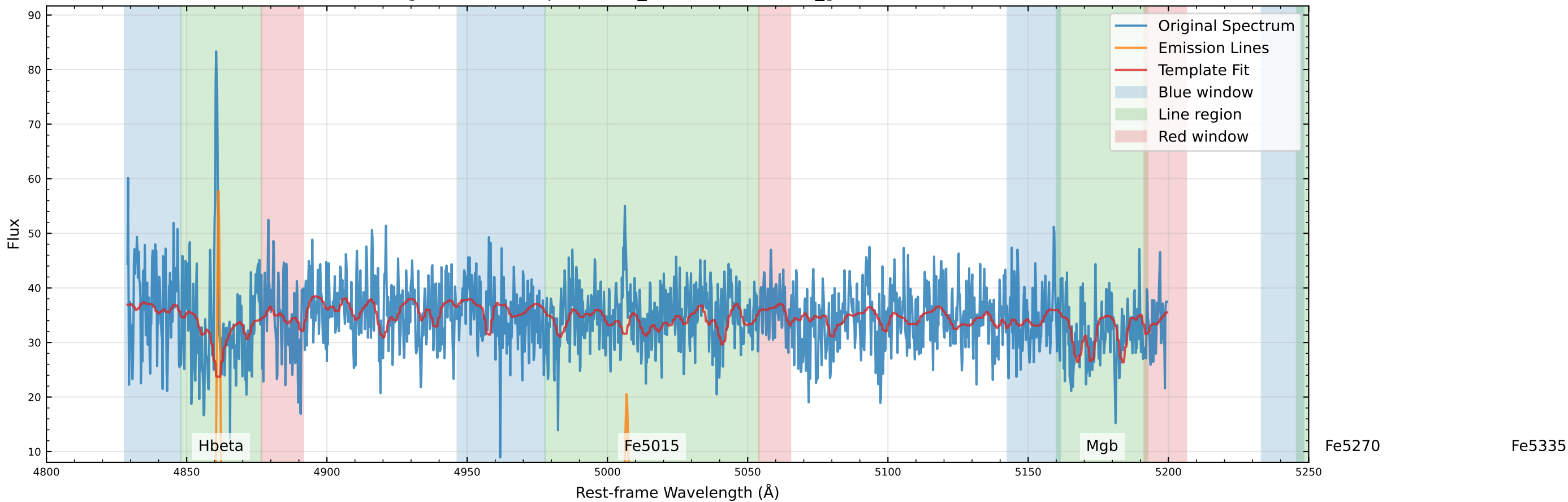
Original Data Comparison (v_star=-56.8 km/s, v_gas=-46.0 km/s)
