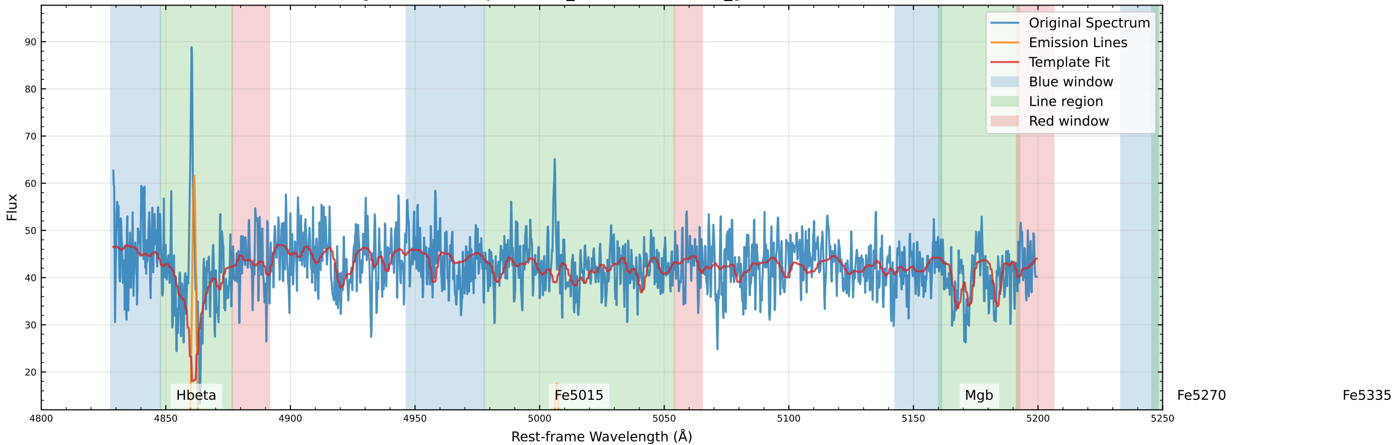
Original Data Comparison (v_star=-74.4 km/s, v_gas=-63.0 km/s)
