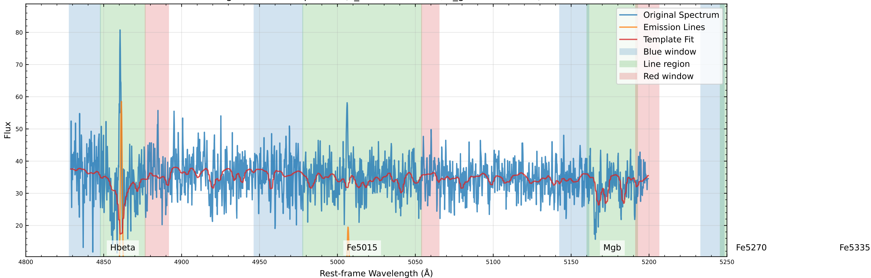
Original Data Comparison (v_star=-70.6 km/s, v_gas=-49.1 km/s)
