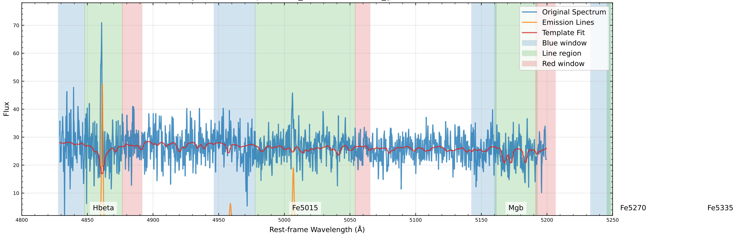
Original Data Comparison (v_star=-62.7 km/s, v_gas=-45.6 km/s)
