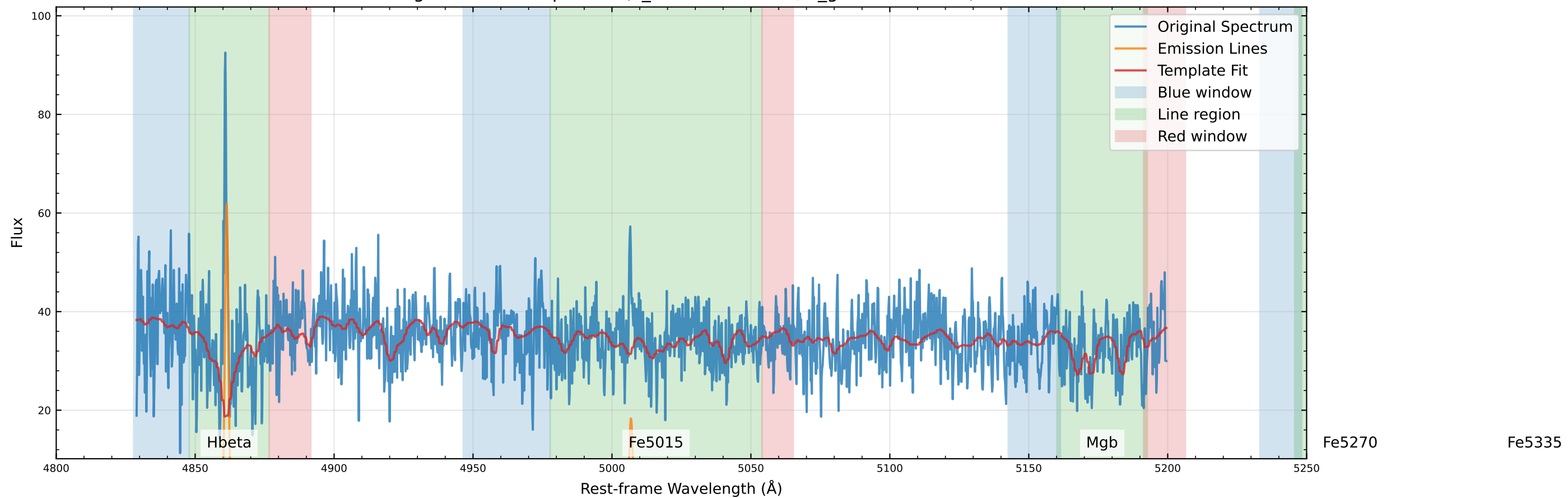
Original Data Comparison (v_star=-43.4 km/s, v_gas=-27.6 km/s)
