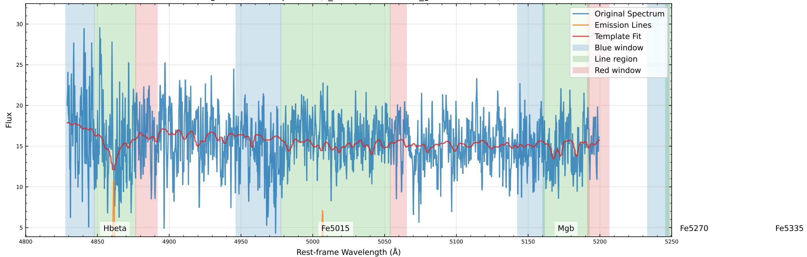
Original Data Comparison (v_star=-78.6 km/s, v_gas=-72.6 km/s)
