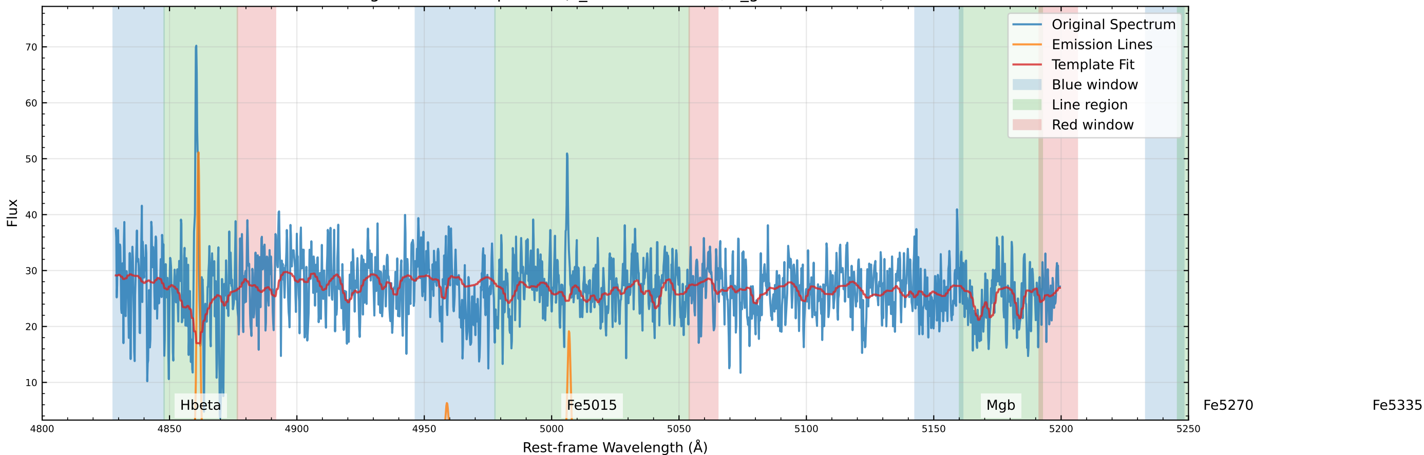
Original Data Comparison (v_star=-55.3 km/s, v_gas=-46.2 km/s)
