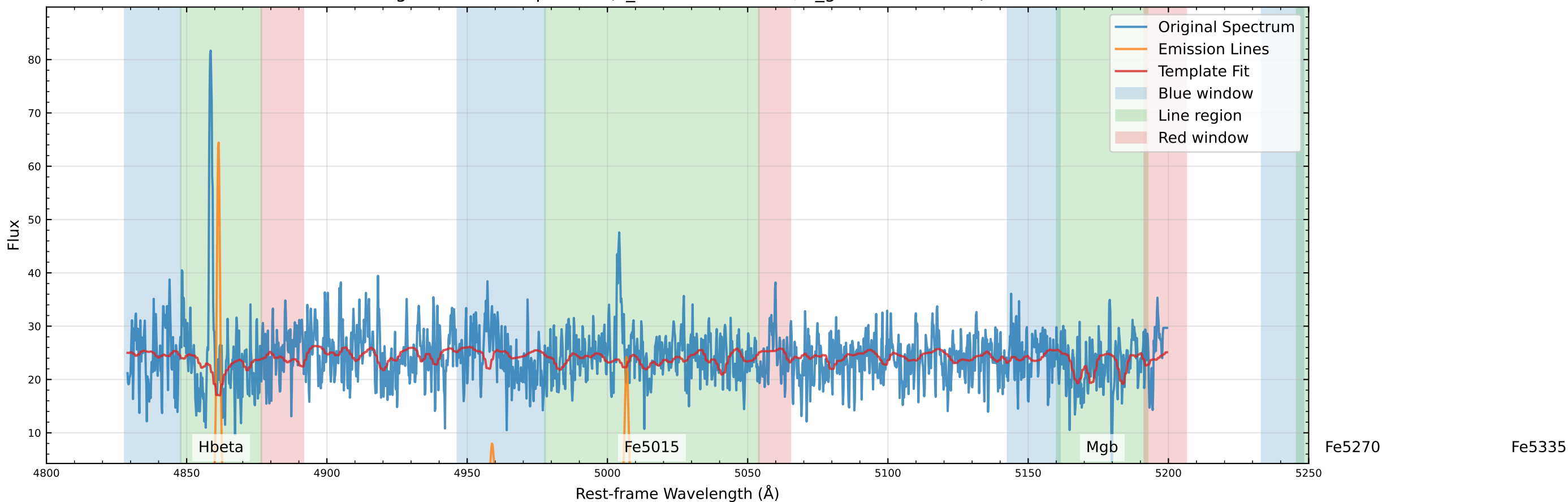
Original Data Comparison (v_star=-170.2 km/s, v_gas=-168.2 km/s)
