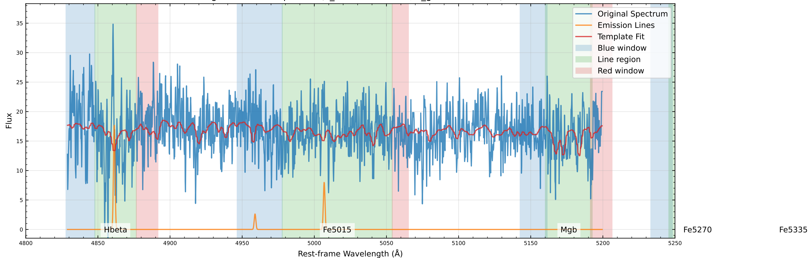
Original Data Comparison (v_star=-61.6 km/s, v_gas=-57.8 km/s)
