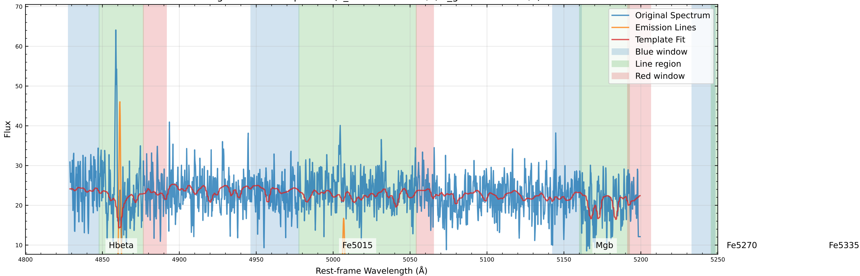
Original Data Comparison (v_star=-148.6 km/s, v_gas=-154.2 km/s)
