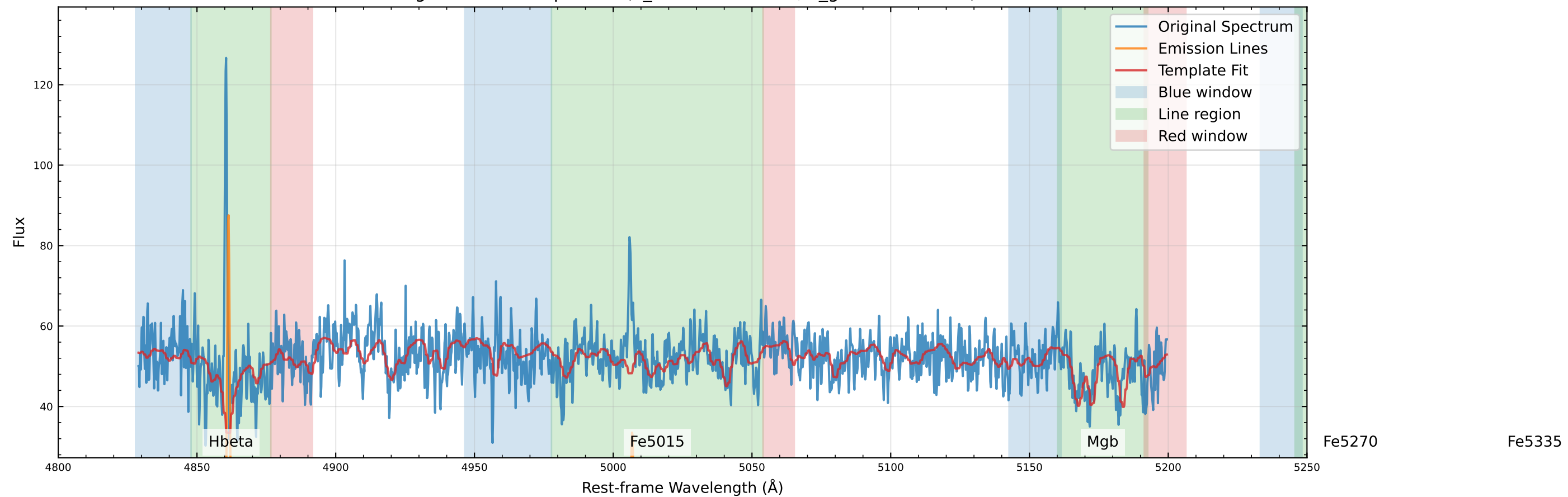
Original Data Comparison (v_star=-53.5 km/s, v_gas=-55.8 km/s)
