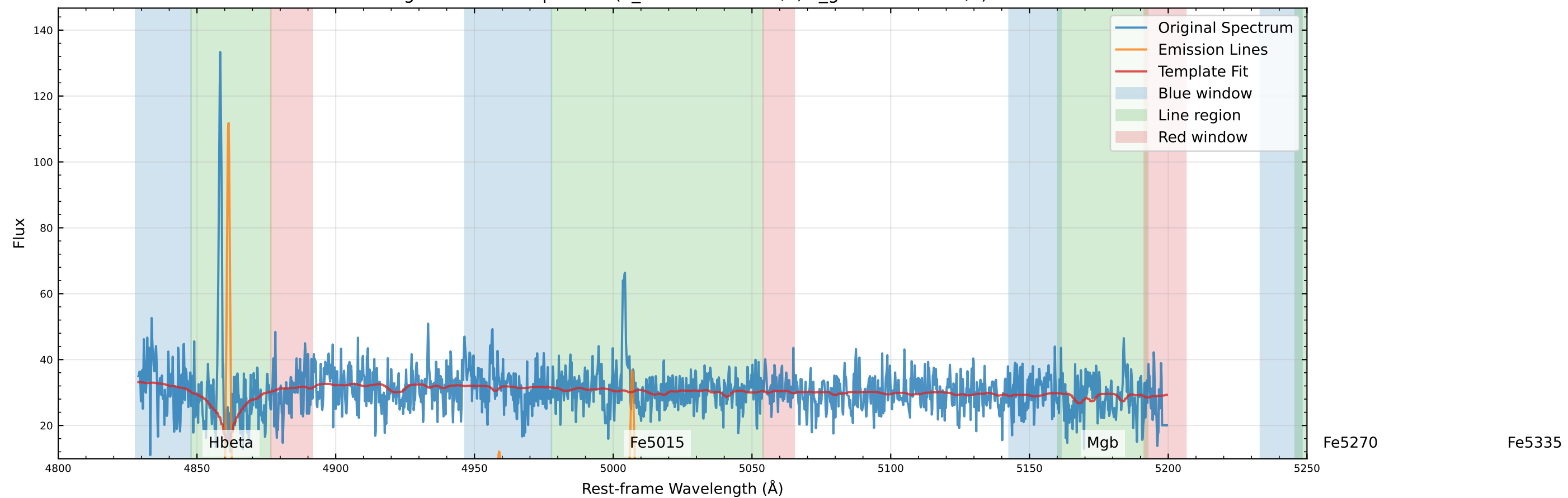
Original Data Comparison (v_star=-203.0 km/s, v_gas=-182.0 km/s)
