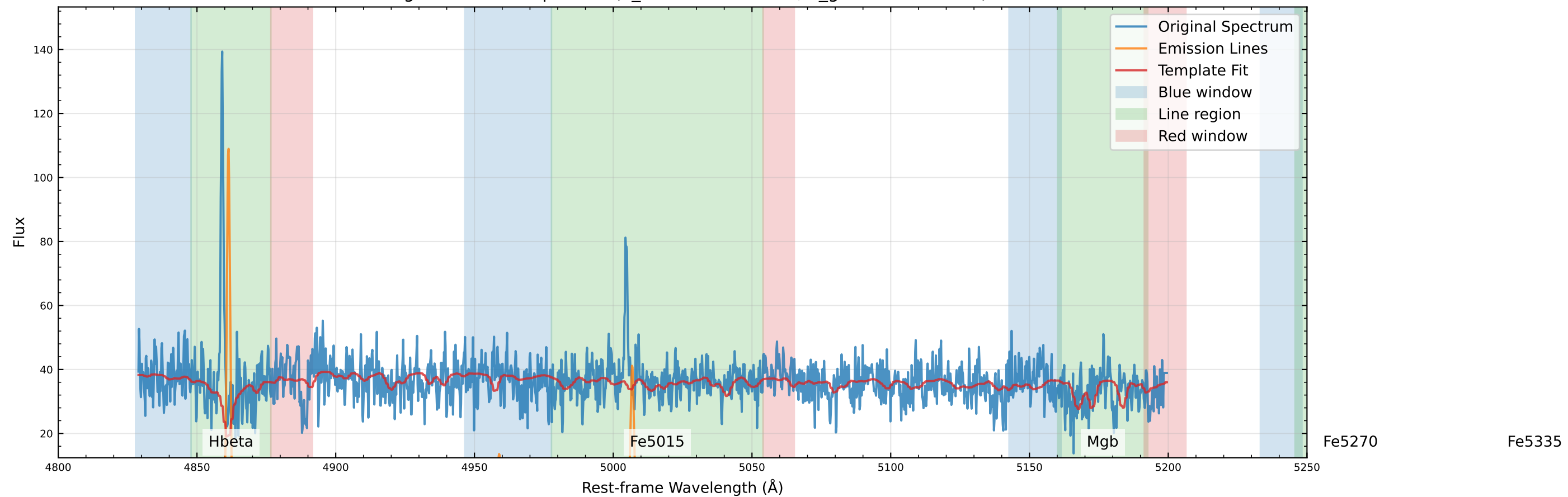
Original Data Comparison (v_star=-134.1 km/s, v_gas=-138.5 km/s)
