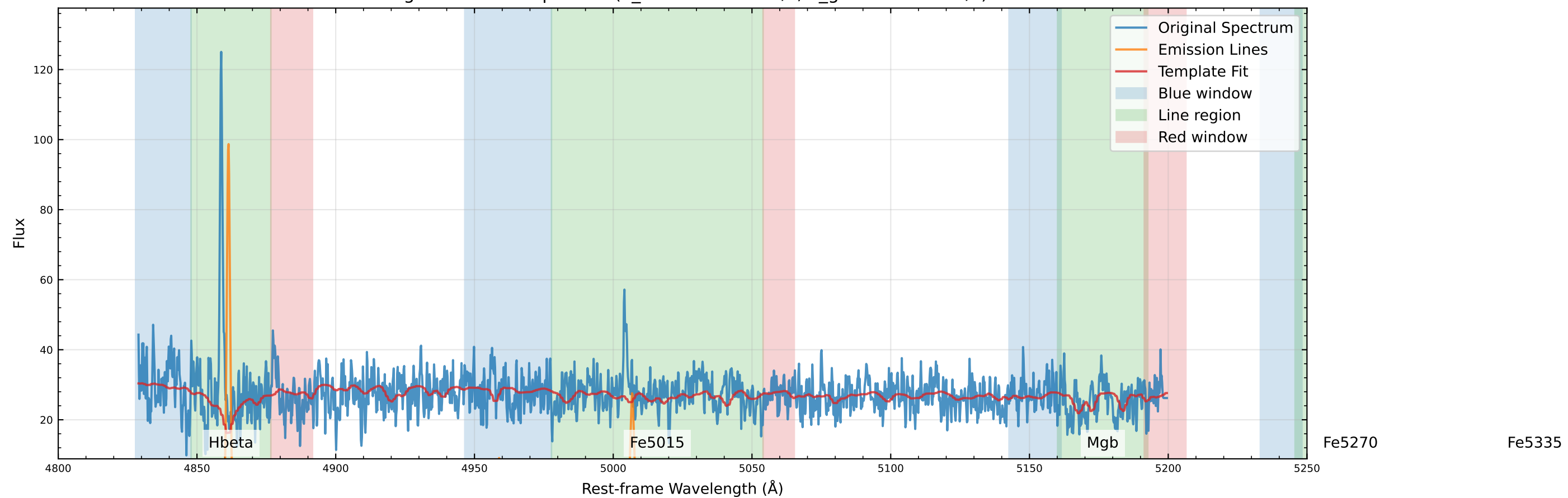
Original Data Comparison (v_star=-153.8 km/s, v_gas=-158.7 km/s)
