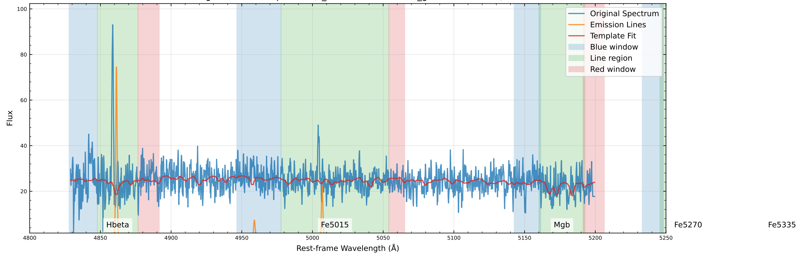
Original Data Comparison (v_star=-167.2 km/s, v_gas=-163.8 km/s)
