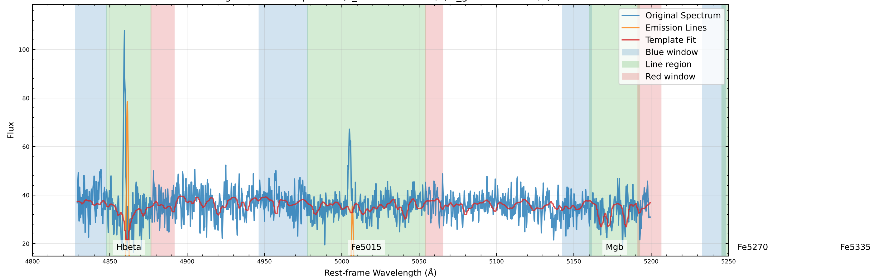
Original Data Comparison (v_star=-101.2 km/s, v_gas=-115.0 km/s)
