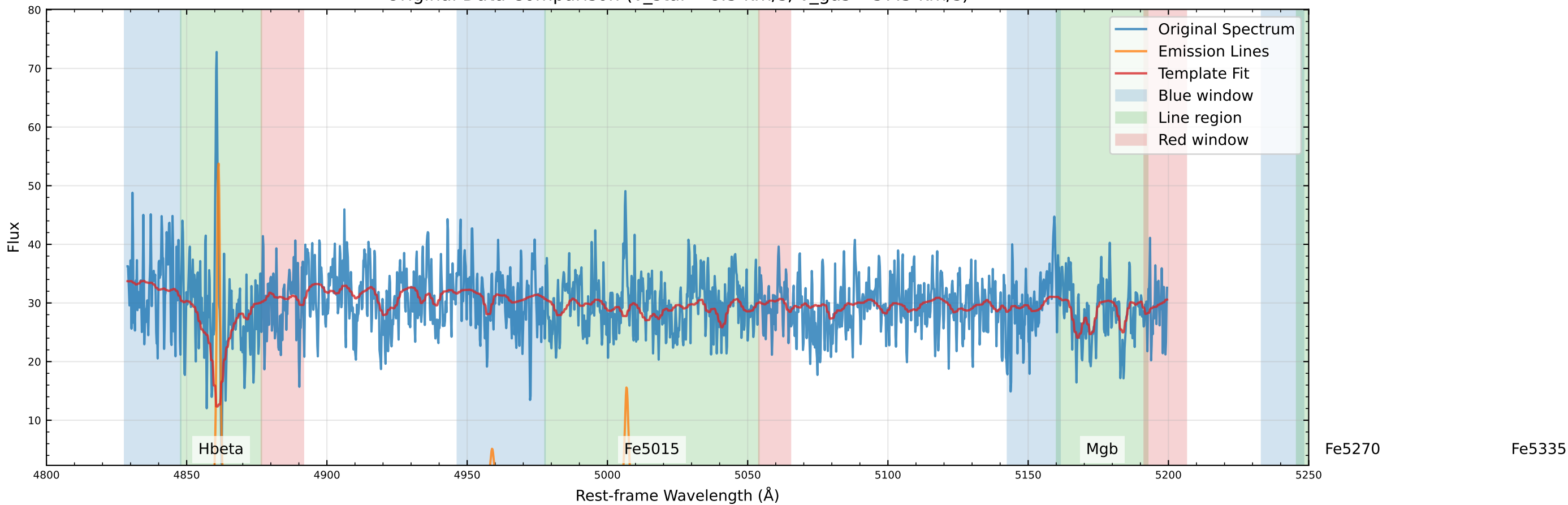
Original Data Comparison (v_star=-8.3 km/s, v_gas=-37.5 km/s)
