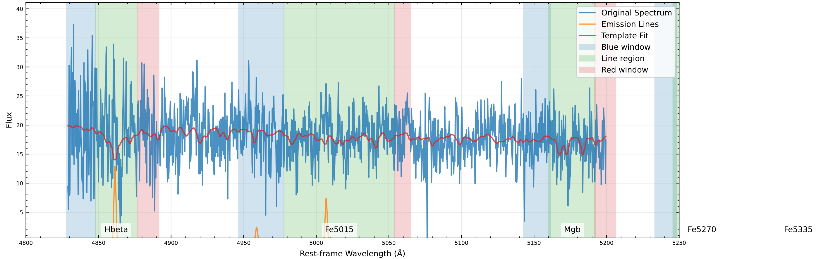
Original Data Comparison (v_star=40.8 km/s, v_gas=-26.7 km/s)
