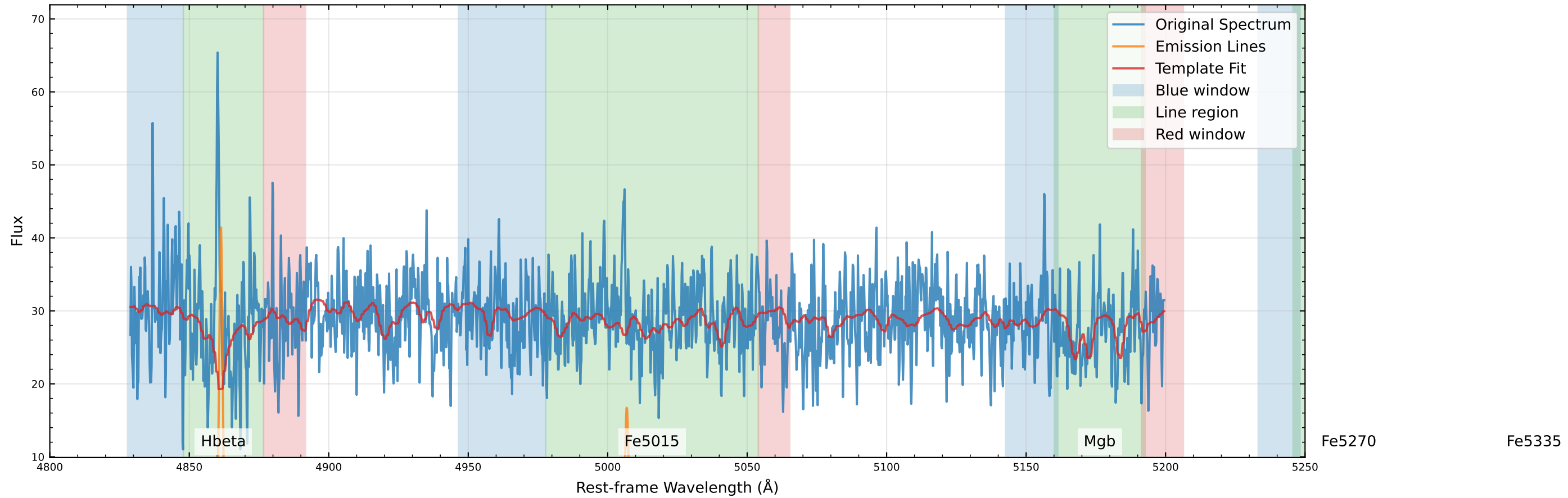
Original Data Comparison (v_star=-60.9 km/s, v_gas=-69.5 km/s)
