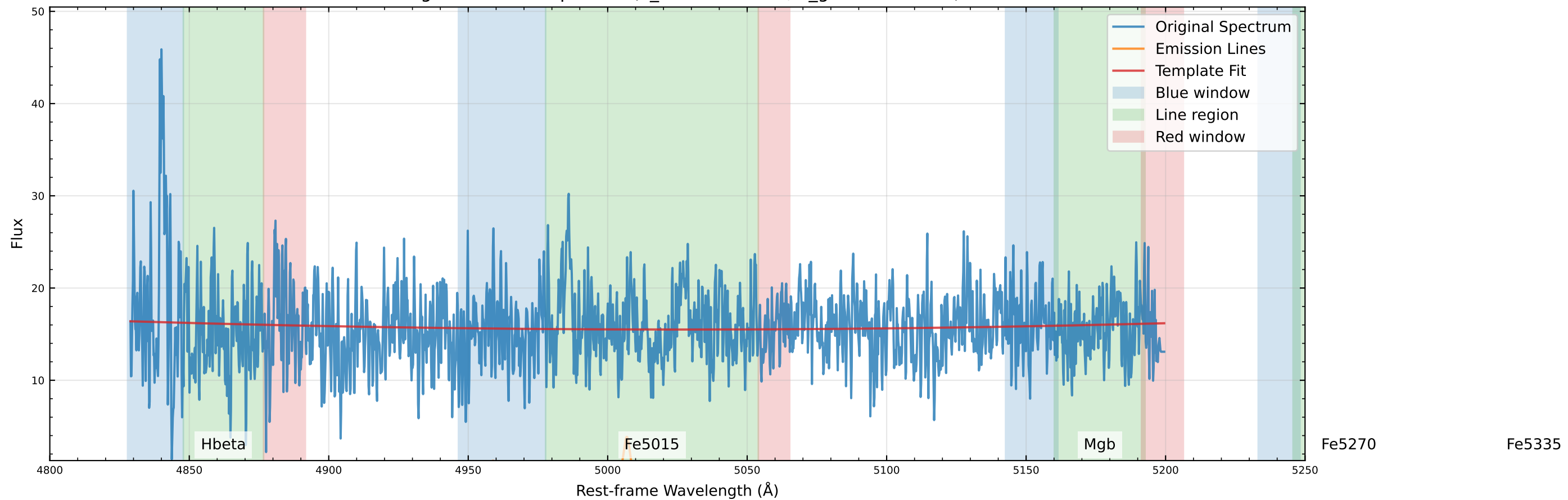
Original Data Comparison (v_star=0.0 km/s, v_gas=91.1 km/s)
