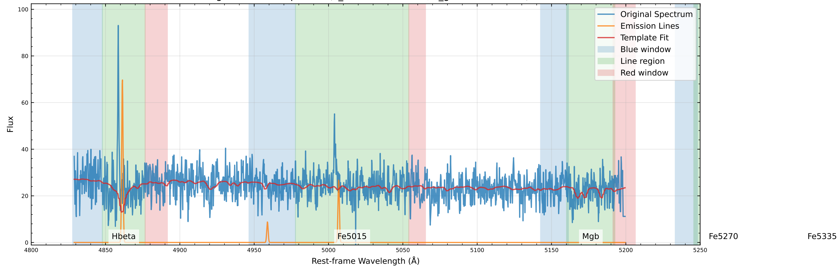
Original Data Comparison (v_star=-153.6 km/s, v_gas=-168.5 km/s)
