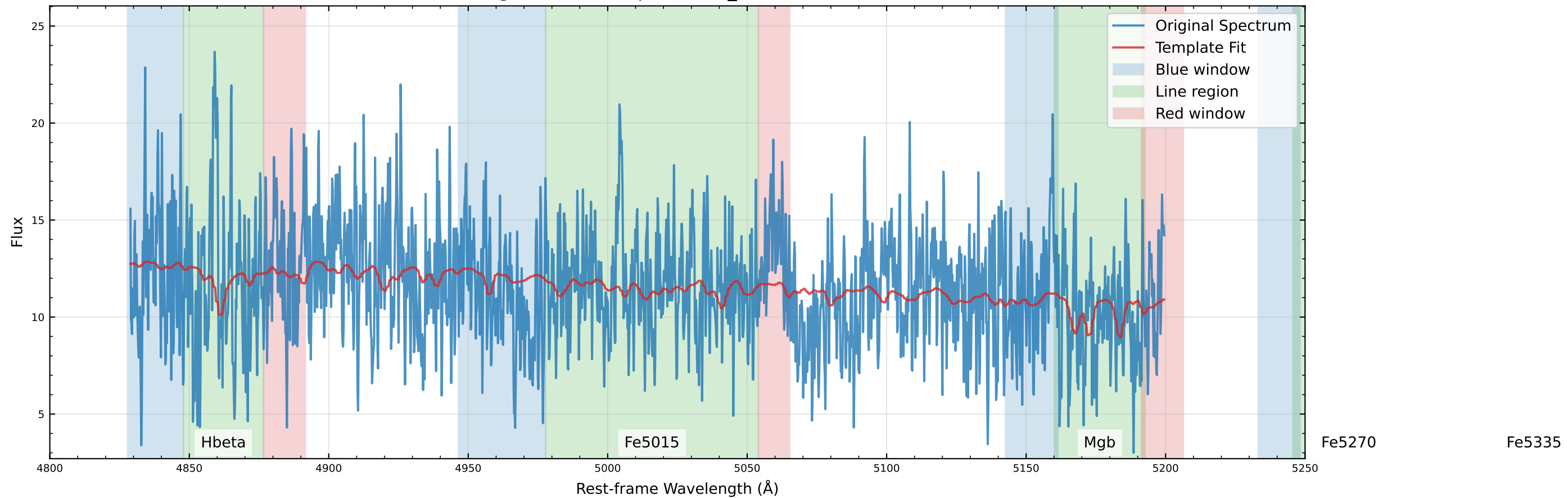
Original Data Comparison ( v_{\text{star}}=38.9 km/s)
