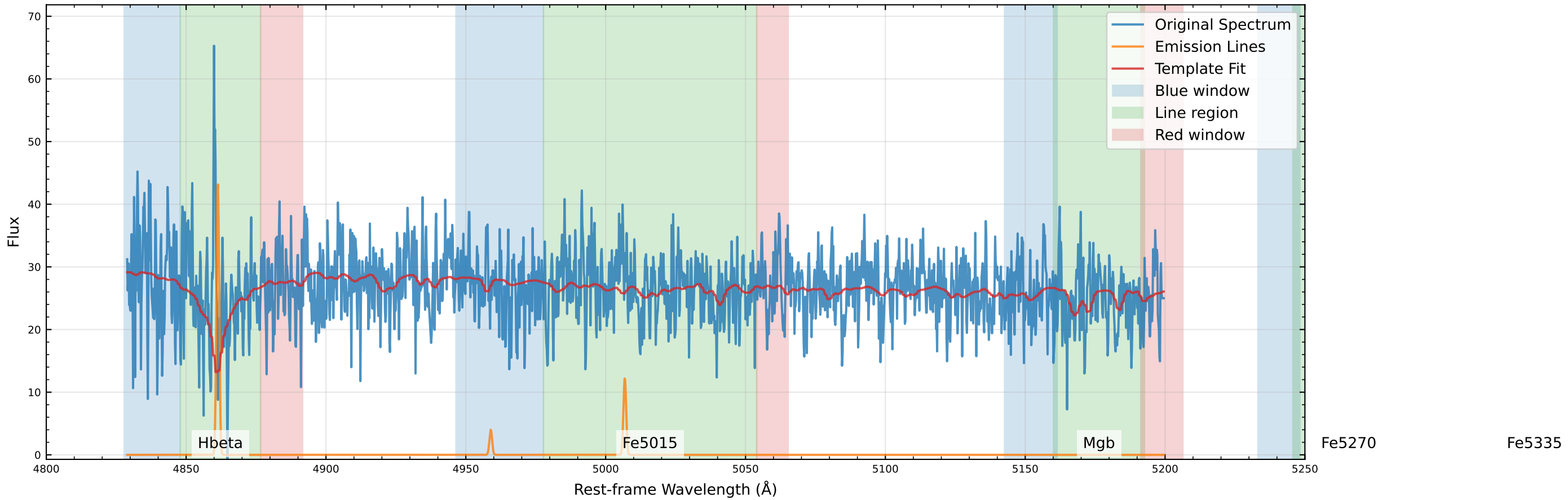
Original Data Comparison (v_star=-84.0 km/s, v_gas=-74.9 km/s)
