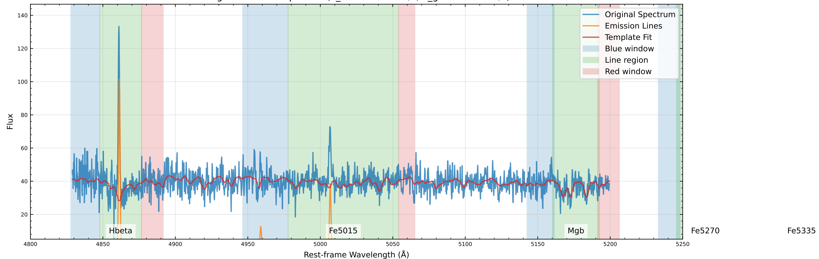
Original Data Comparison (v_star=-23.4 km/s, v_gas=-18.3 km/s)
