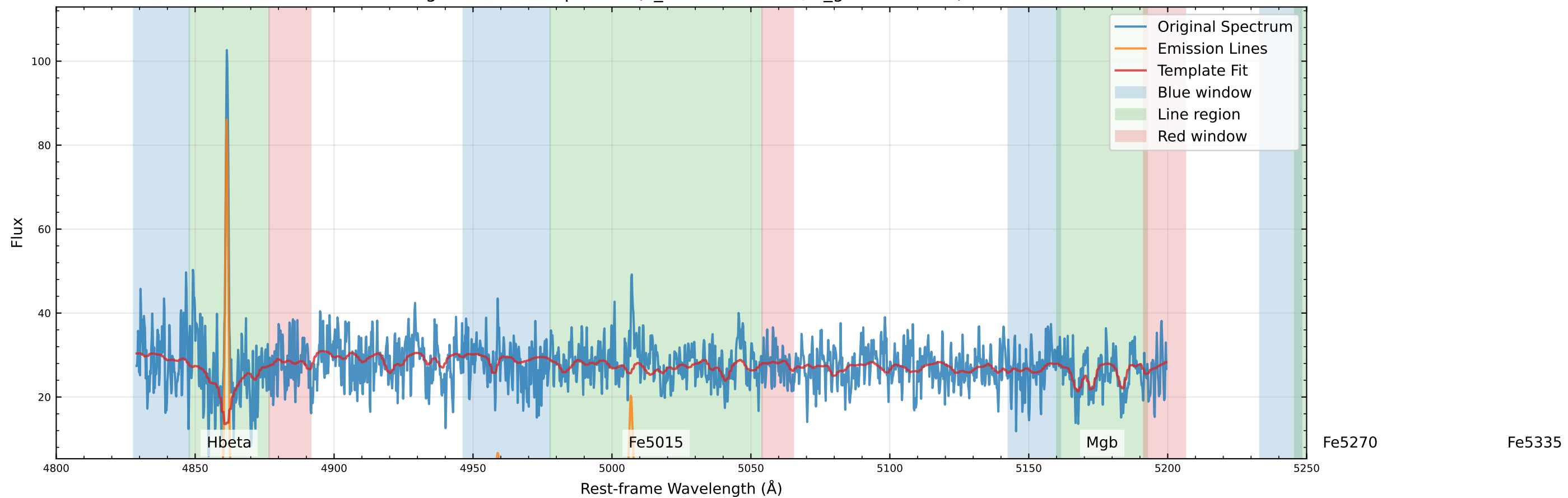
Original Data Comparison (v_star=27.9 km/s, v_gas=9.7 km/s)
