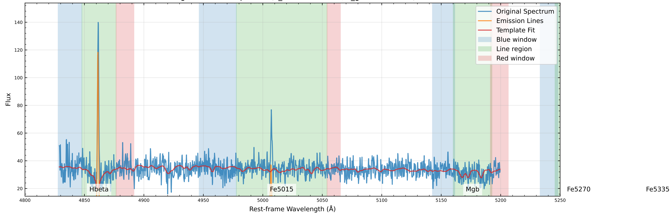
Original Data Comparison (v_star=36.5 km/s, v_gas=16.8 km/s)
