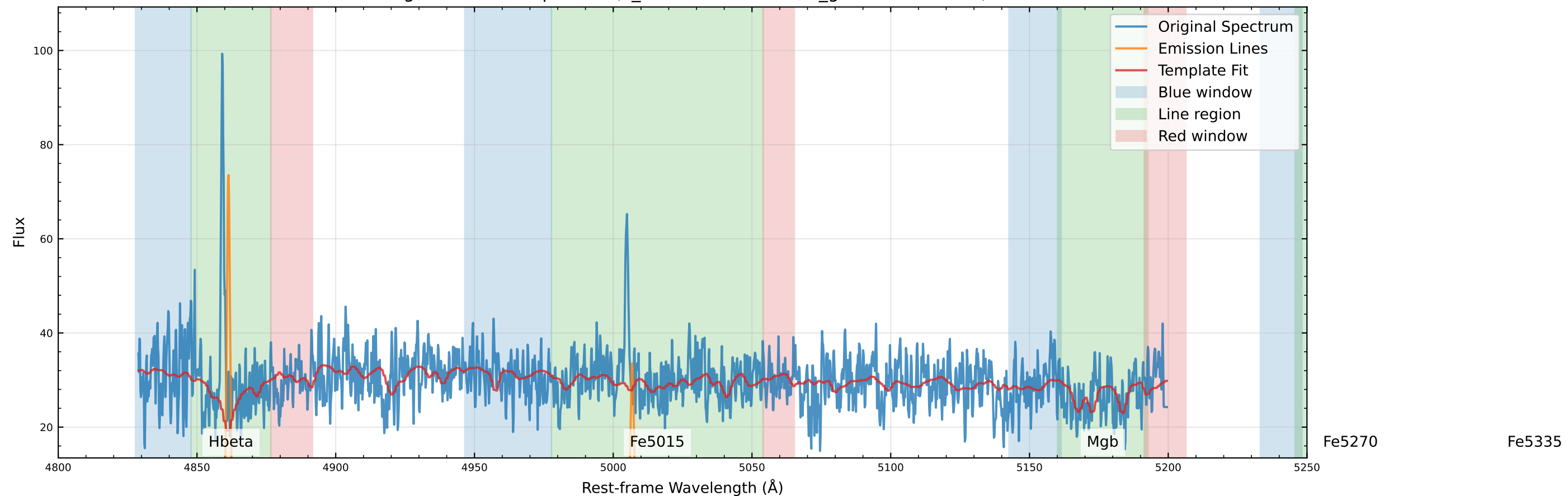
Original Data Comparison (v_star=-116.9 km/s, v_gas=-129.3 km/s)
