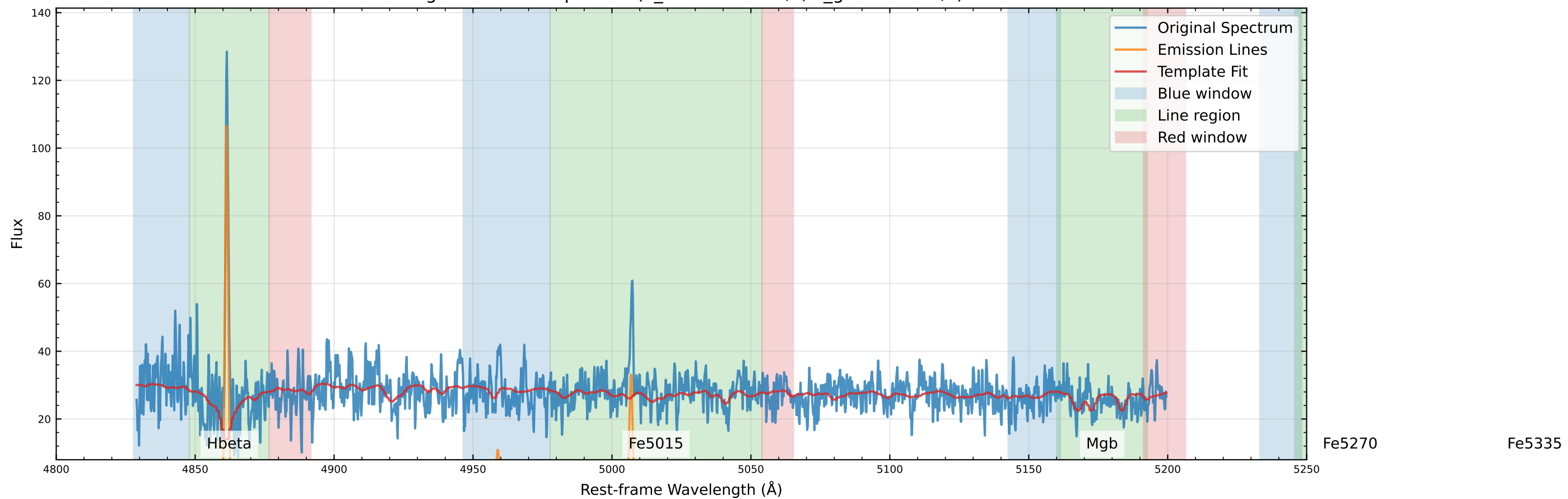
Original Data Comparison (v_star=16.9 km/s, v_gas=7.7 km/s)
