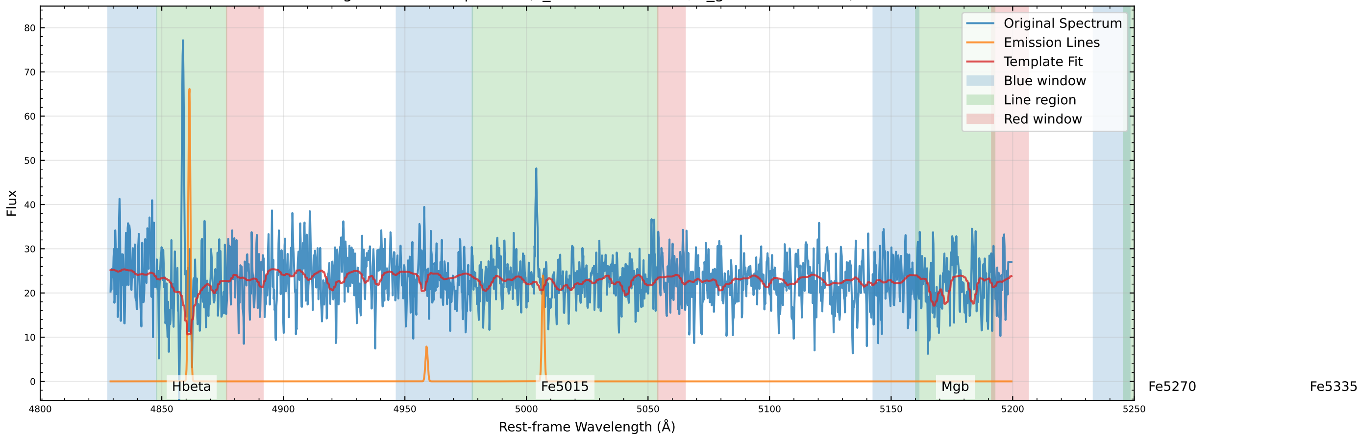
Original Data Comparison (v_star=-156.6 km/s, v_gas=-162.5 km/s)
