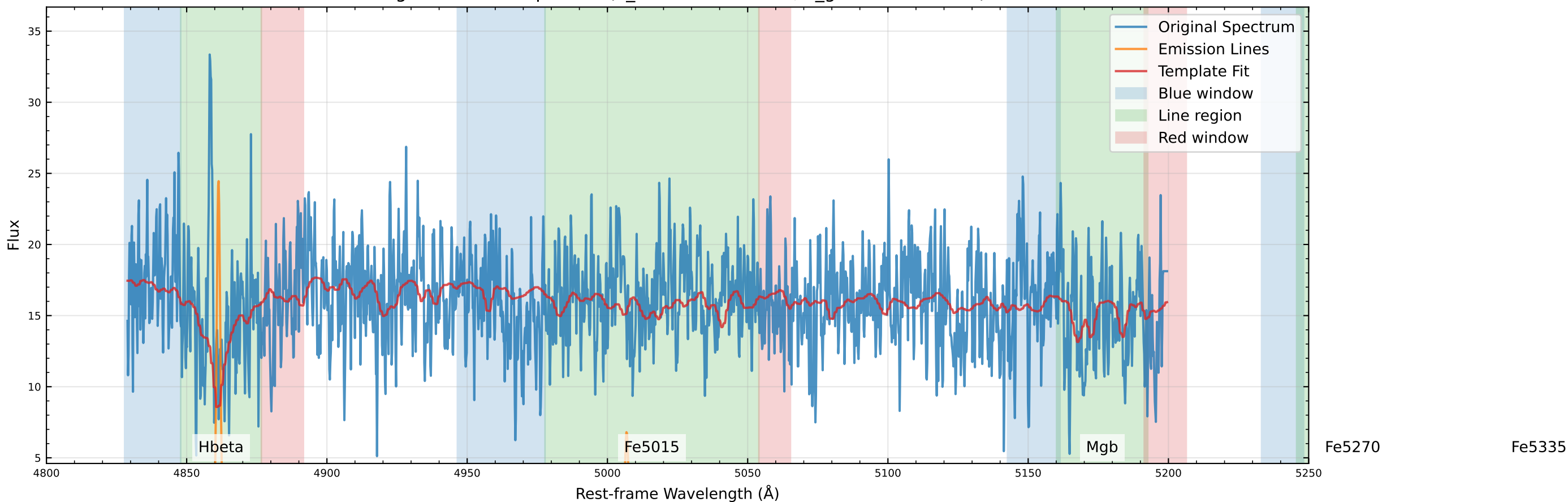
Original Data Comparison (v_star=-176.9 km/s, v_gas=-178.0 km/s)
