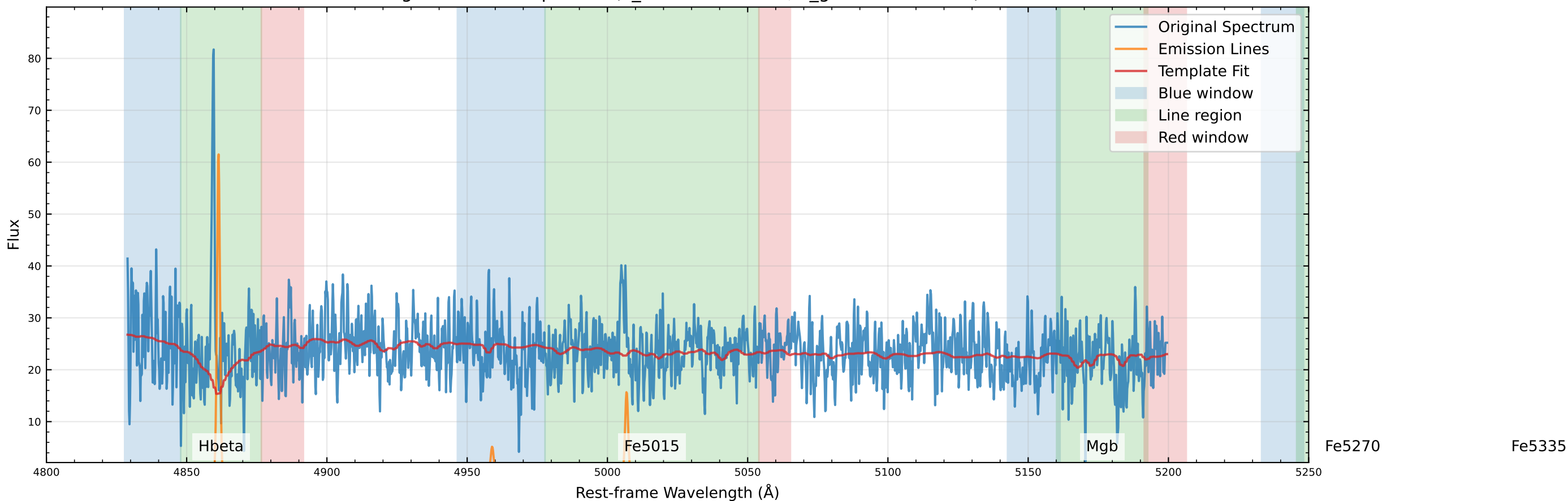
Original Data Comparison (v_star=-82.3 km/s, v_gas=-116.1 km/s)
