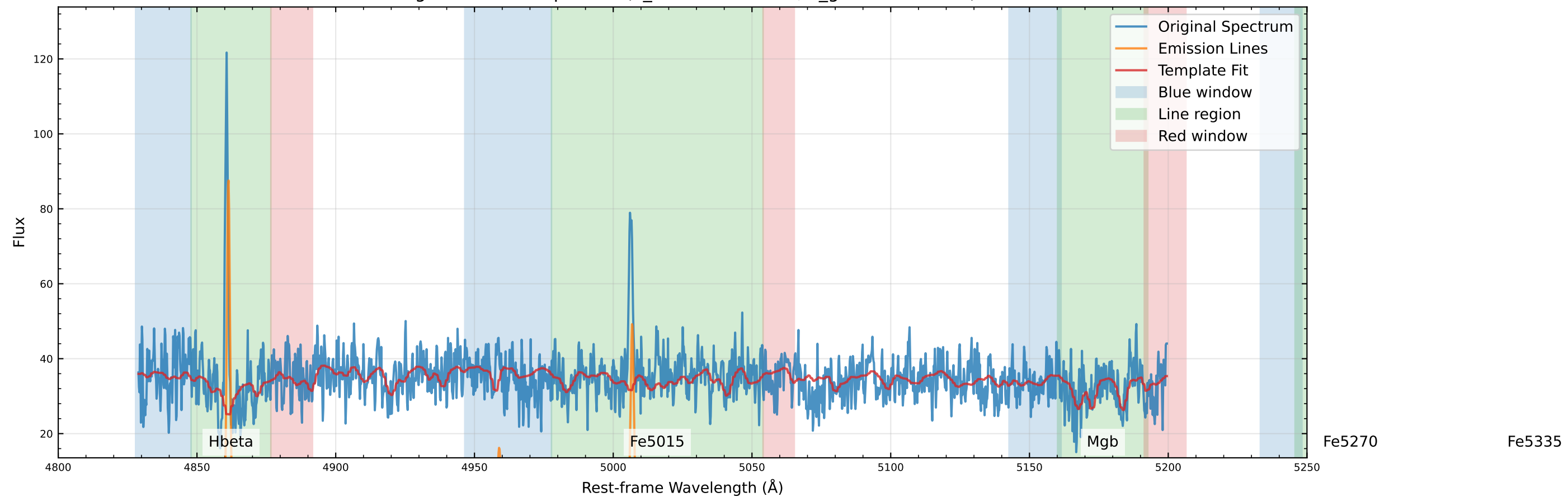
Original Data Comparison (v_star=-25.1 km/s, v_gas=-39.5 km/s)
