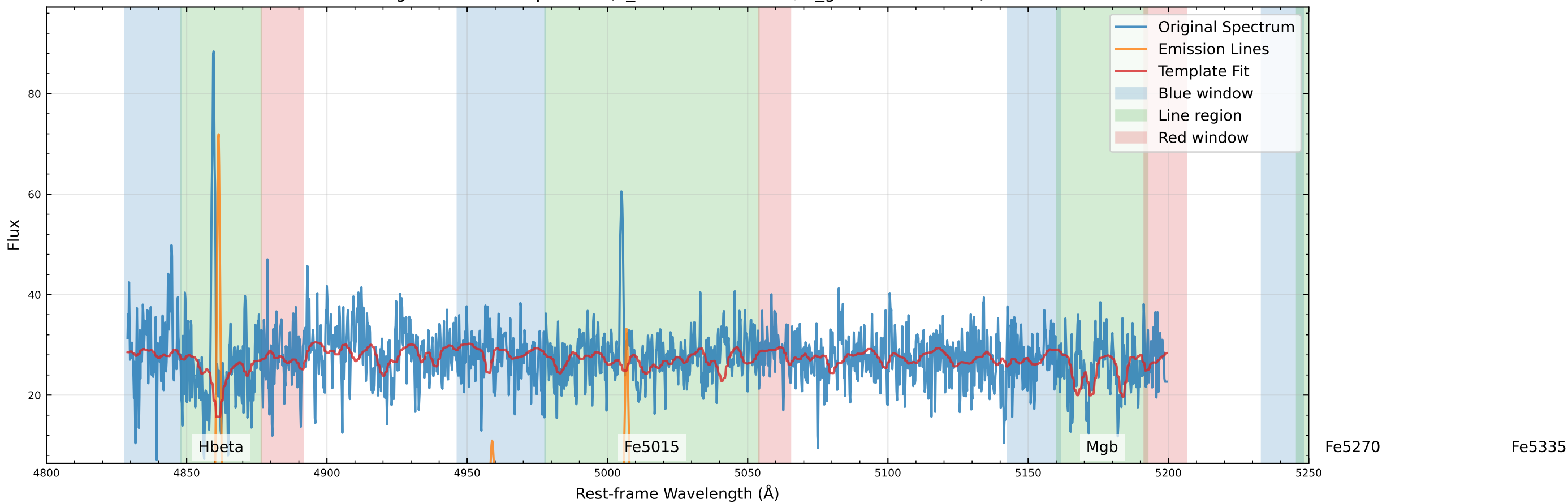
Original Data Comparison (v_star=-113.1 km/s, v_gas=-111.3 km/s)
