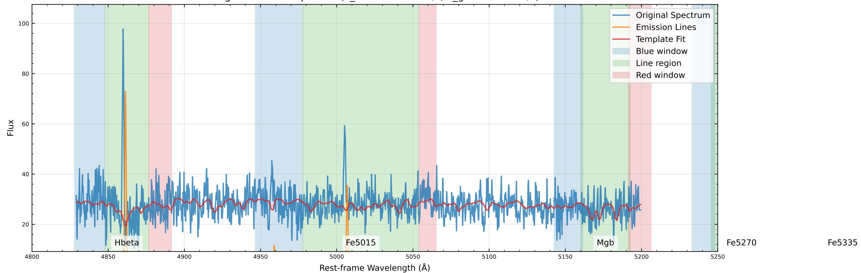
Original Data Comparison (v_star=-127.7 km/s, v_gas=-96.5 km/s)
