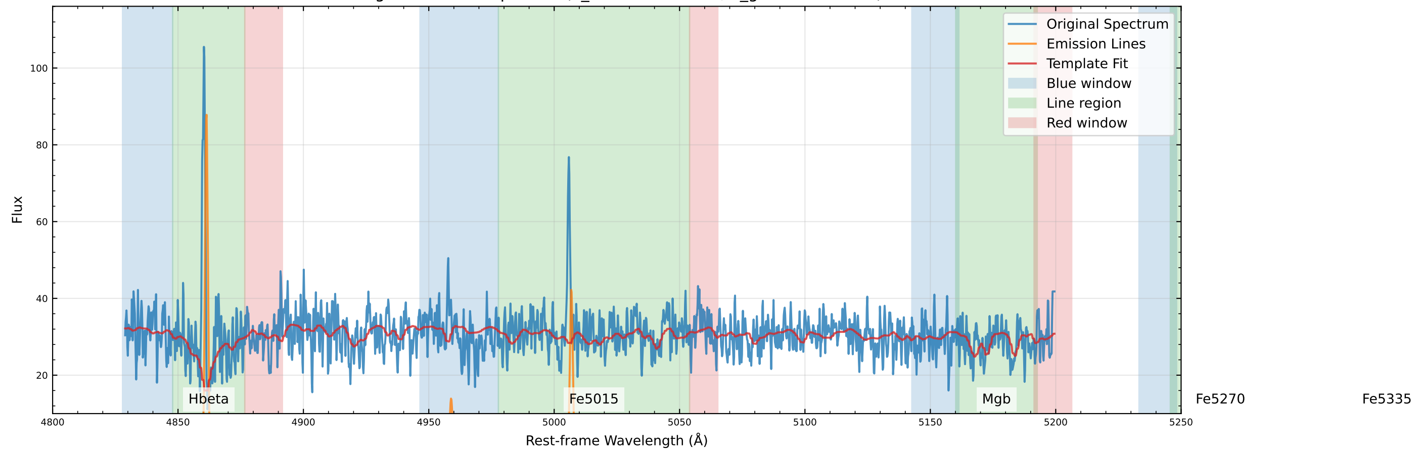
Original Data Comparison (v_star=-97.1 km/s, v_gas=-67.2 km/s)
