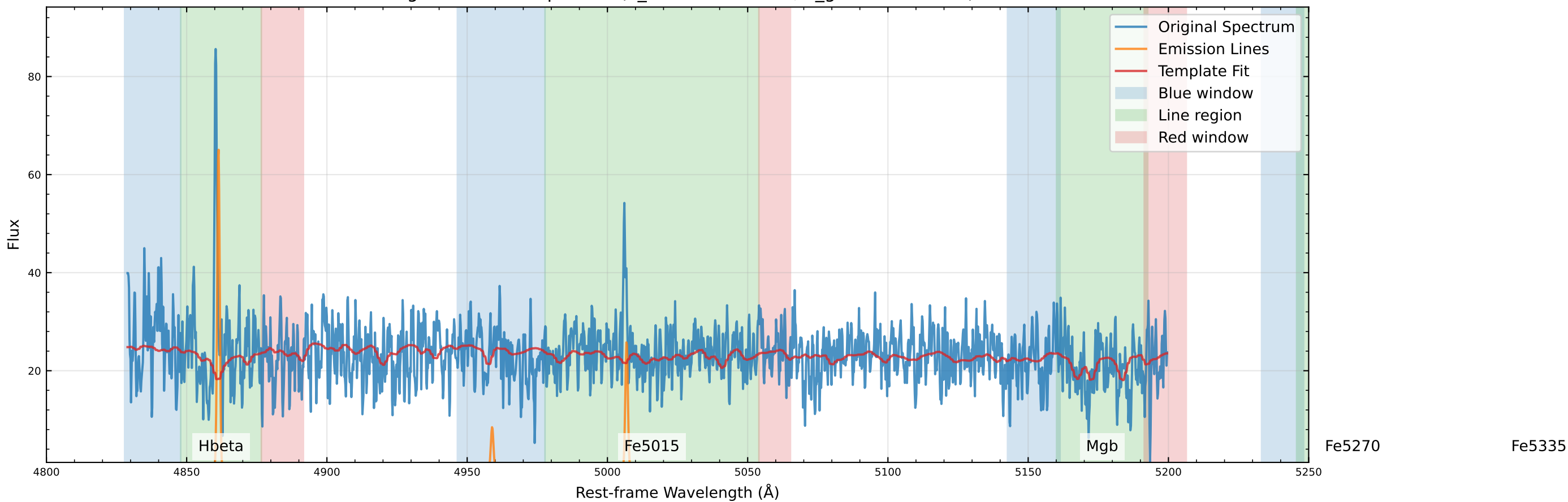
Original Data Comparison (v_star=-35.3 km/s, v_gas=-56.3 km/s)
