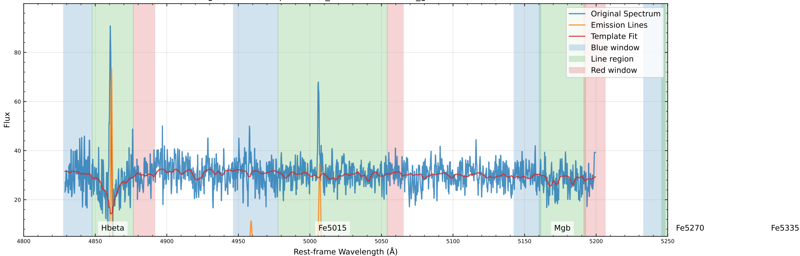
Original Data Comparison (v_star=-89.1 km/s, v_gas=-52.8 km/s)
