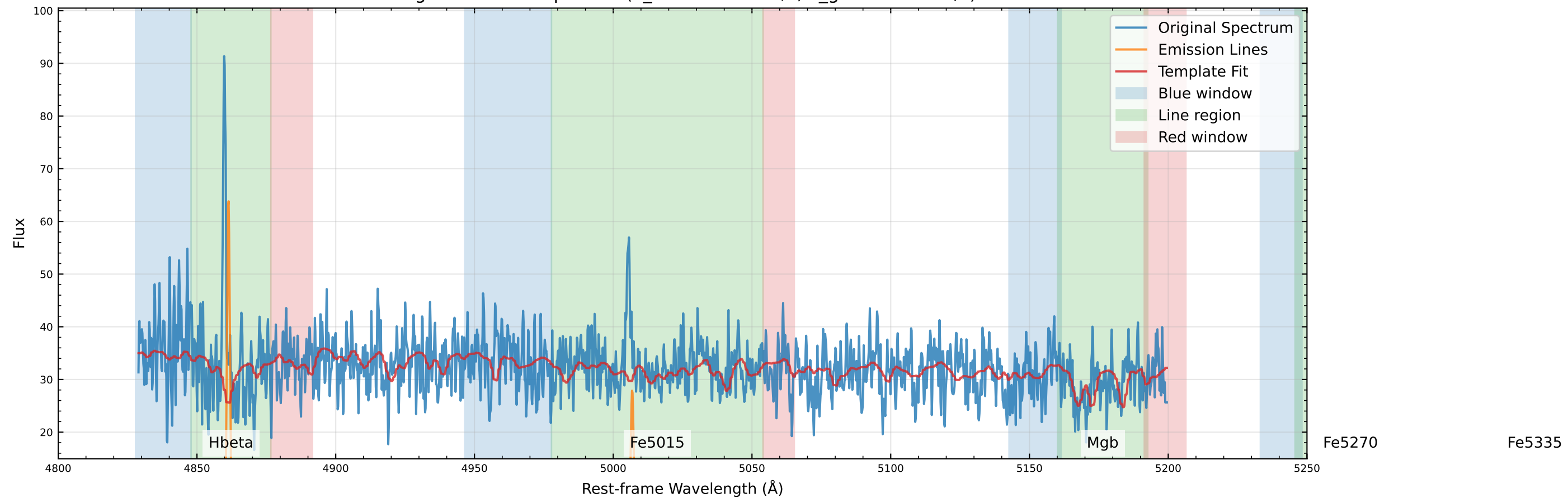
Original Data Comparison (v_star=-79.1 km/s, v_gas=-89.2 km/s)
