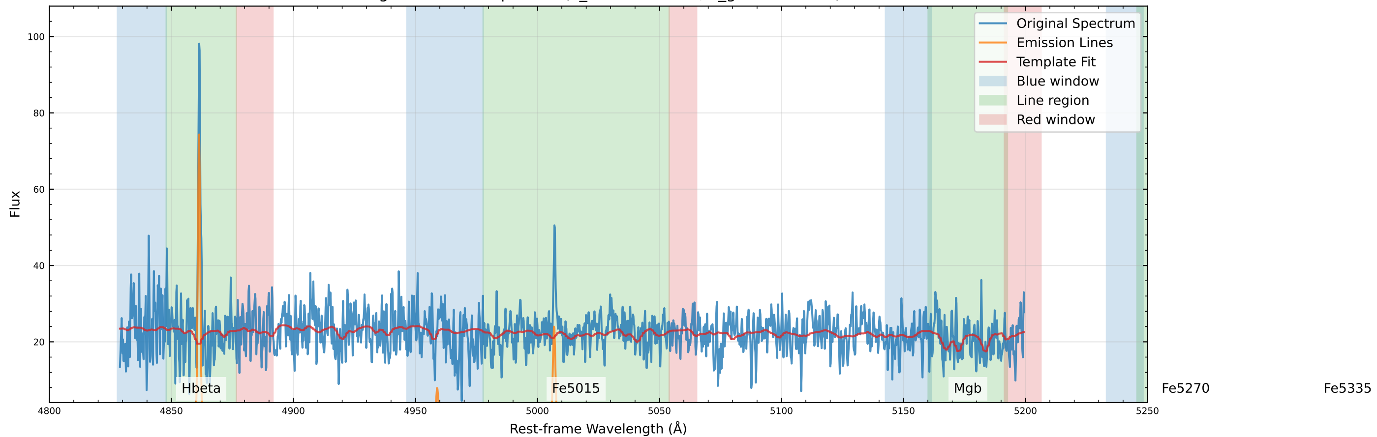
Original Data Comparison (v_star=7.3 km/s, v_gas=8.6 km/s)
