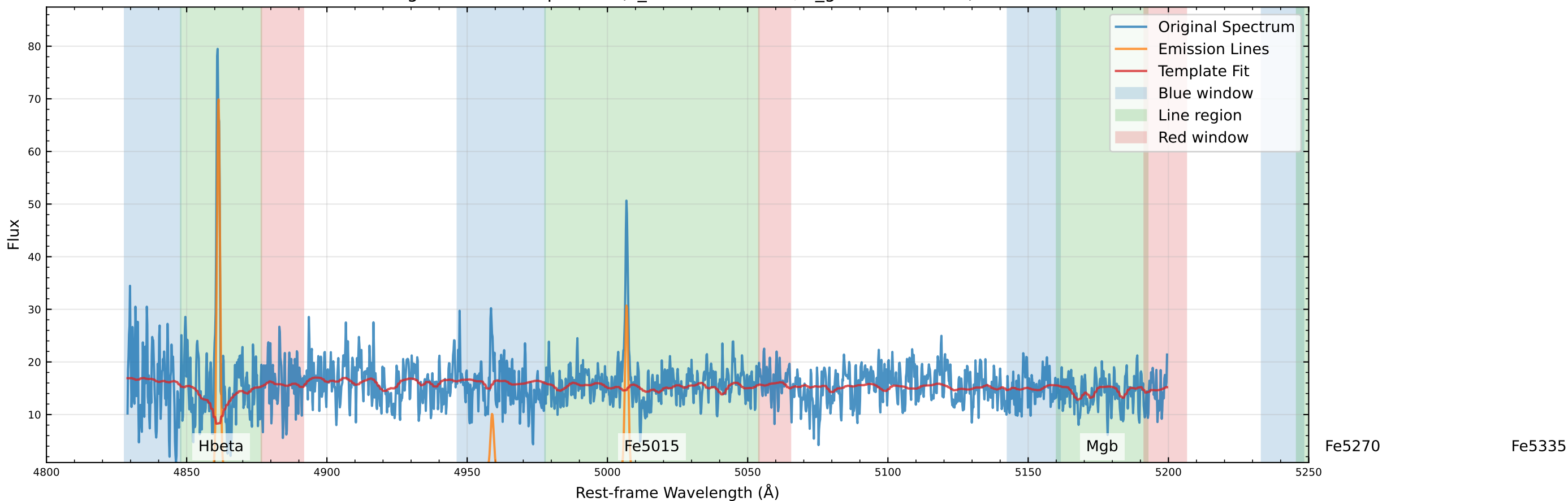
Original Data Comparison (v_star=-22.4 km/s, v_gas=-10.9 km/s)
