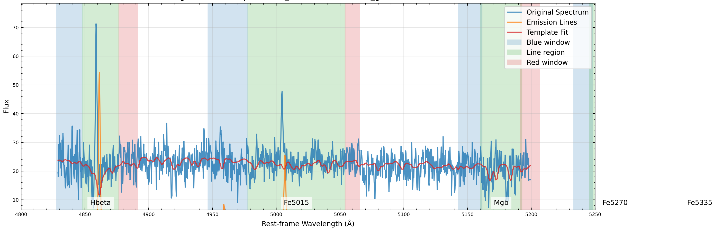
Original Data Comparison (v_star=-166.5 km/s, v_gas=-151.7 km/s)
