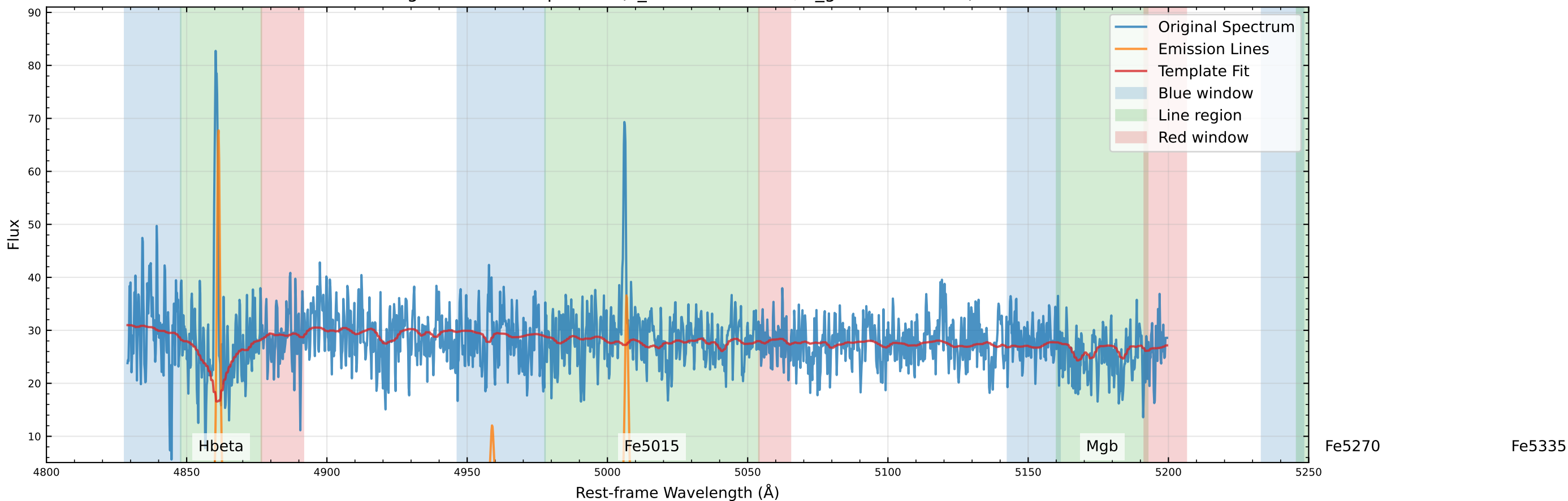
Original Data Comparison (v_star=-70.6 km/s, v_gas=-50.1 km/s)
