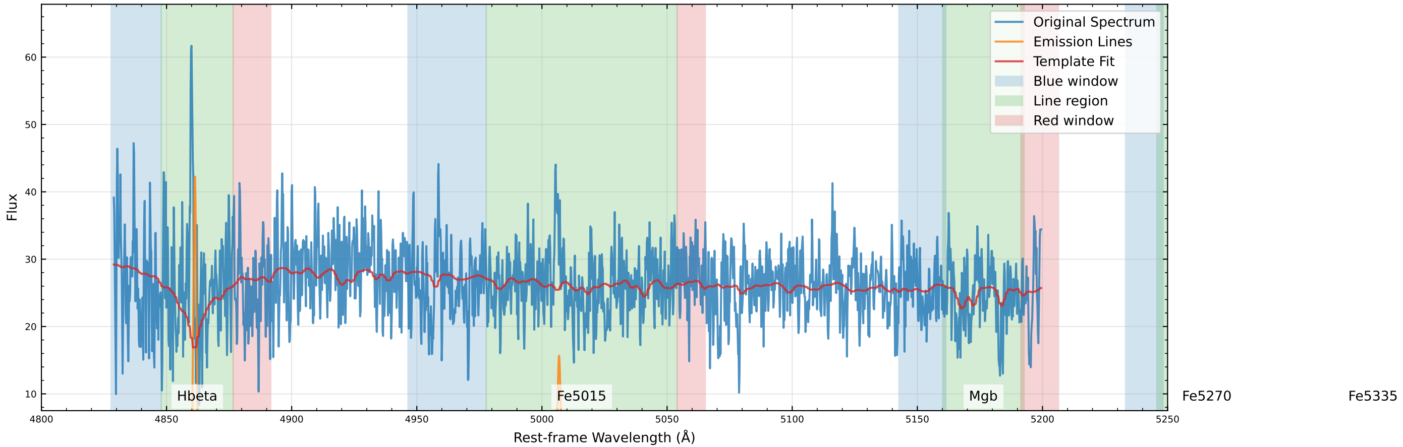
Original Data Comparison (v_star=-57.4 km/s, v_gas=-81.1 km/s)
