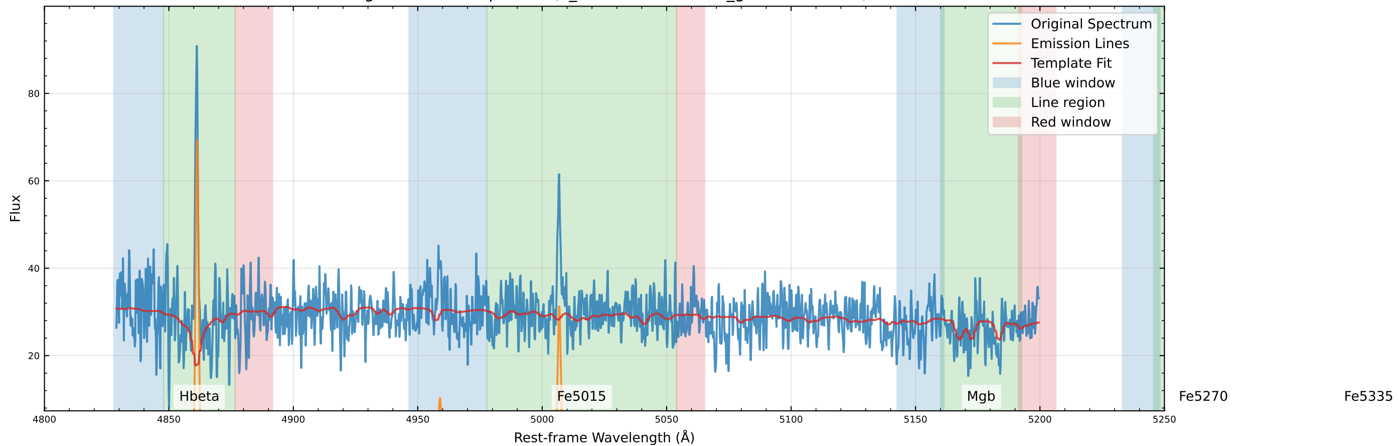
Original Data Comparison (v_star=-34.3 km/s, v_gas=-12.6 km/s)
