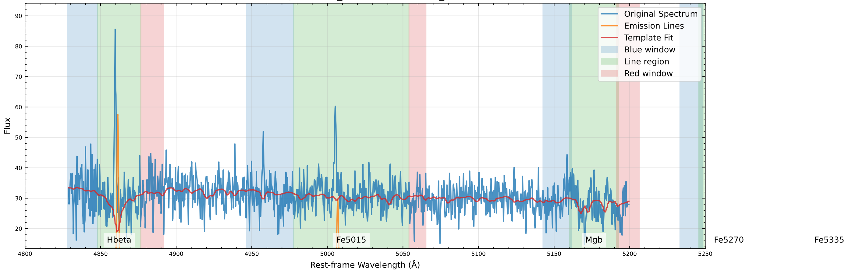
Original Data Comparison (v_star=-101.1 km/s, v_gas=-101.2 km/s)
