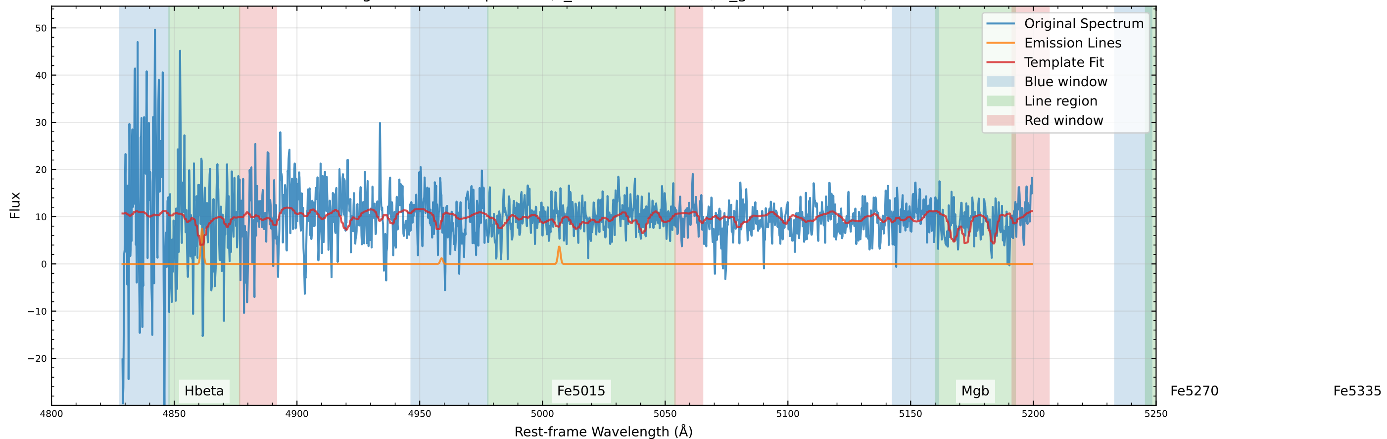
Original Data Comparison (v_star=-102.4 km/s, v_gas=-55.7 km/s)
