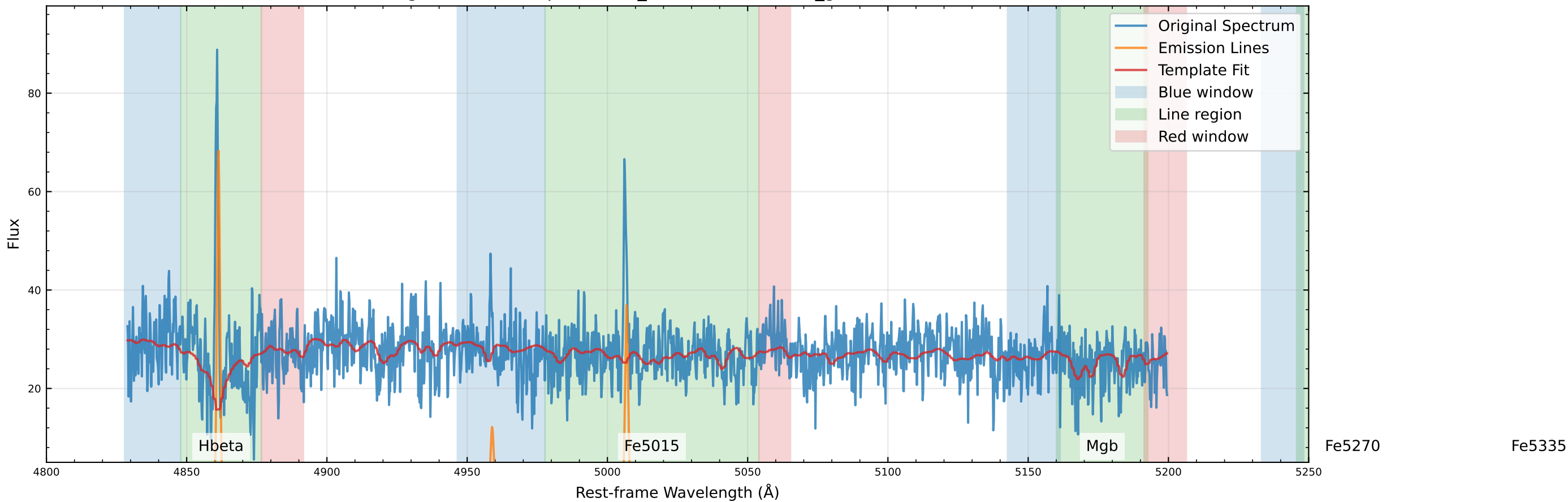
Original Data Comparison (v_star=-20.2 km/s, v_gas=-35.6 km/s)
