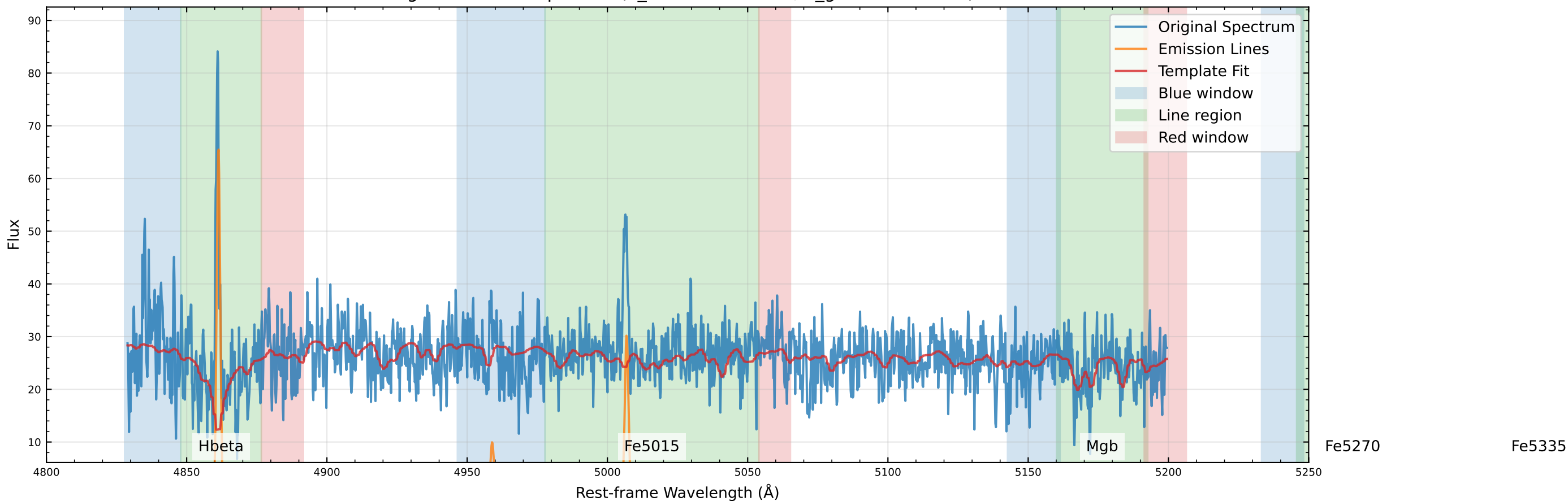
Original Data Comparison (v_star=-44.0 km/s, v_gas=-25.3 km/s)
